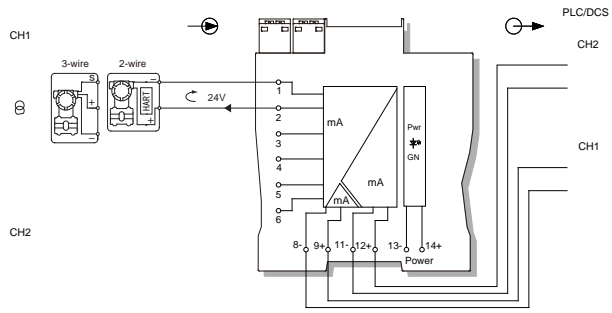
24V DC, double current input, double source current output
